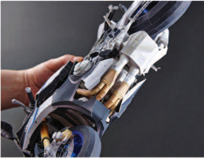
Underside of the Ultra-Realistic YZF-R1M
